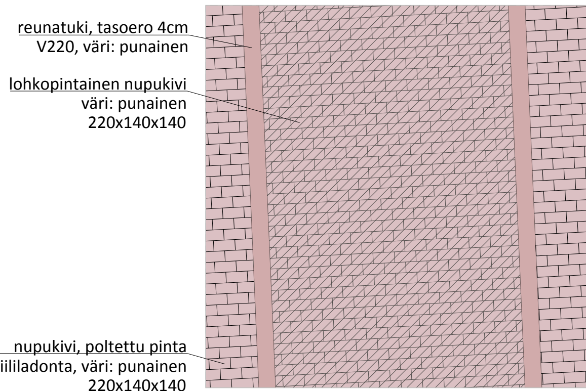
DETALJI 1: Isokadun ajorata
